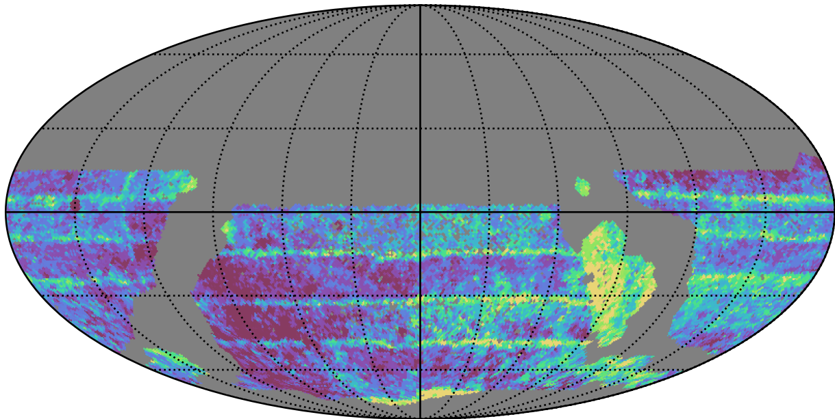
scp_reweight_v3.3_10yrs WFD z band: Median Inter-Night Gap
