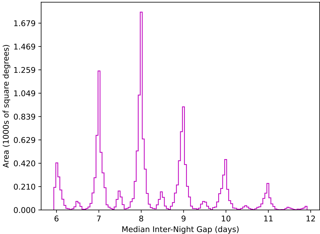
scp_reweight_v3.3_10yrs WFD z band: Median Inter-Night Gap
