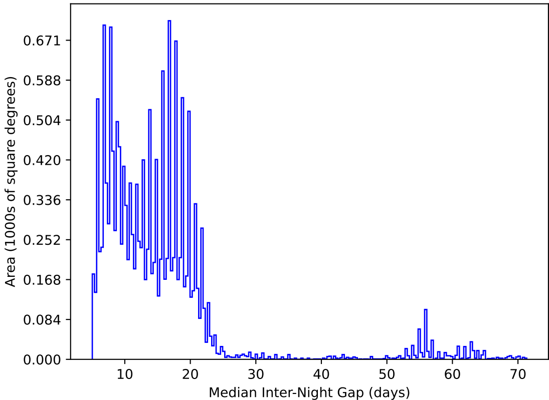
scp_reweight_v3.3_10yrs WFD y band: Median Inter-Night Gap
