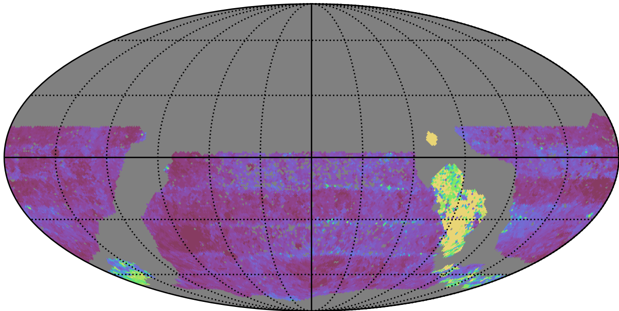
scp_reweight_v3.3_10yrs WFD u band: Median Inter-Night Gap
