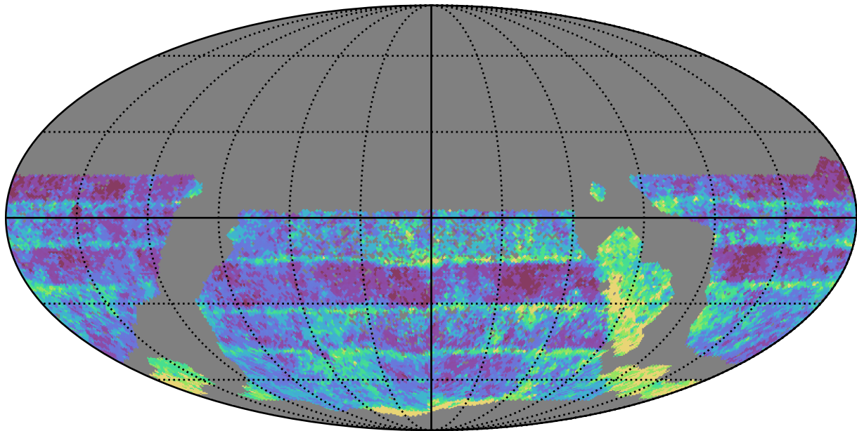
scp_reweight_v3.3_10yrs WFD r band: Median Inter-Night Gap
