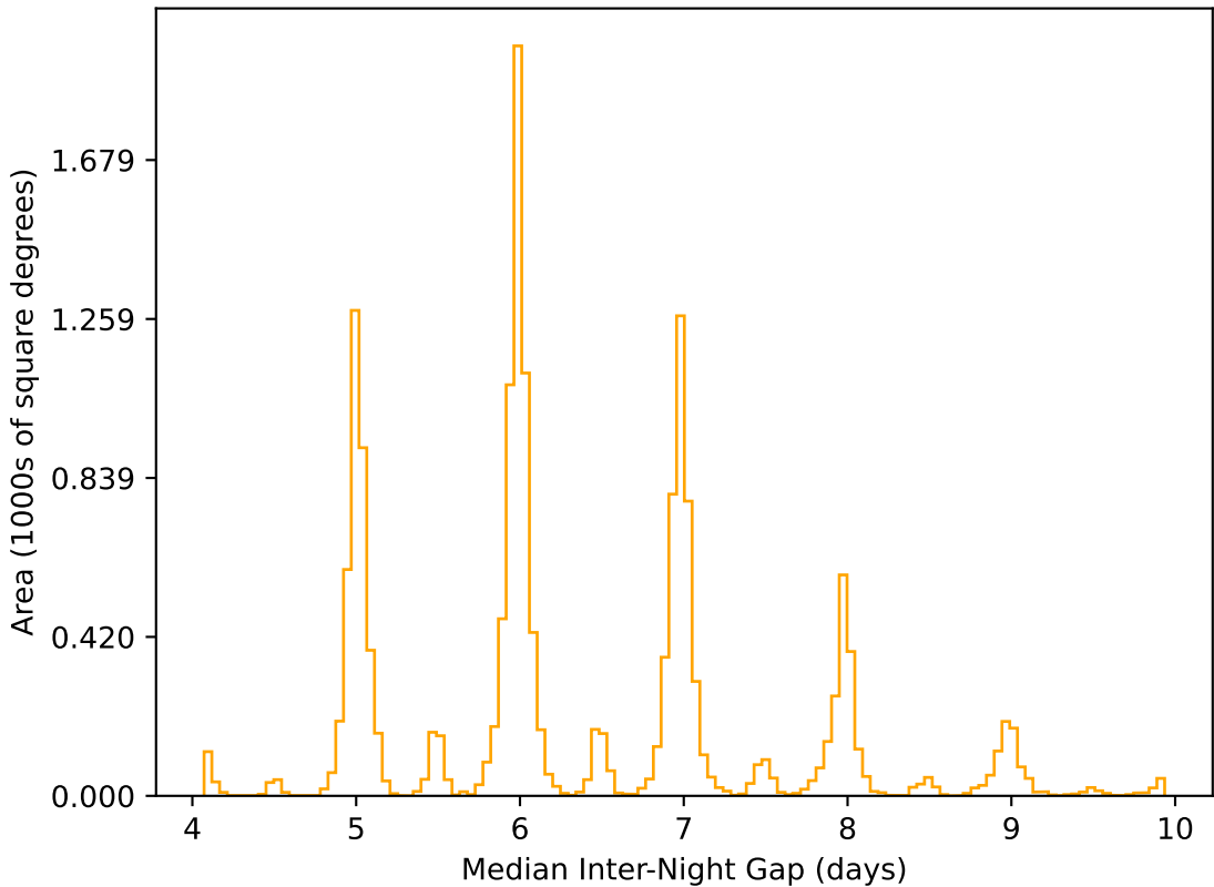
scp_reweight_v3.3_10yrs WFD r band: Median Inter-Night Gap
