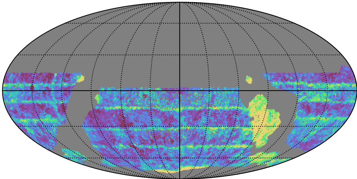
scp_reweight_v3.3_10yrs WFD i band: Median Inter-Night Gap
