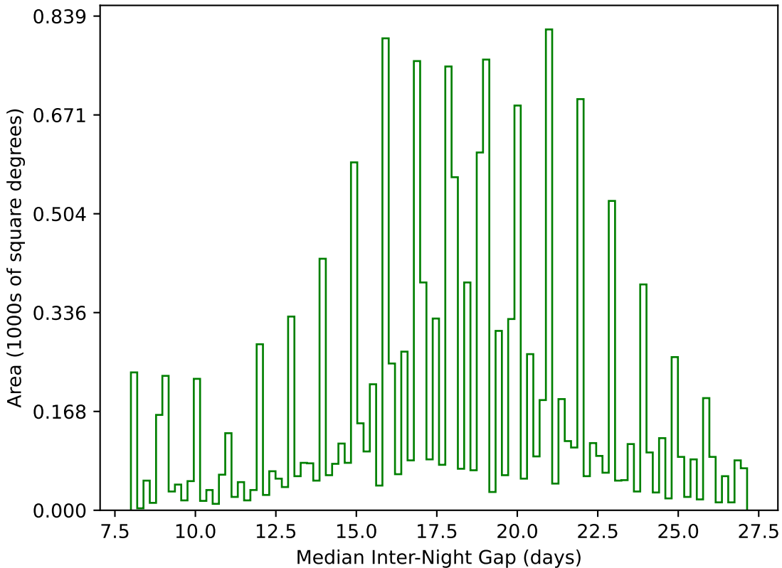
scp_reweight_v3.3_10yrs WFD g band: Median Inter-Night Gap
