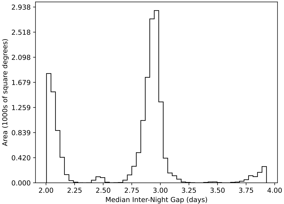
scp_reweight_v3.3_10yrs WFD all bands: Median Inter-Night Gap
