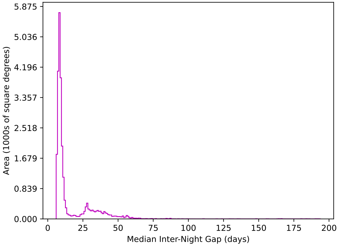
scp_reweight_v3.3_10yrs All sky z band: Median Inter-Night Gap
