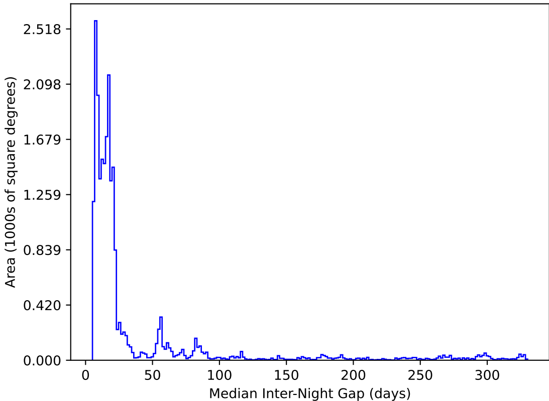
scp_reweight_v3.3_10yrs All sky y band: Median Inter-Night Gap
