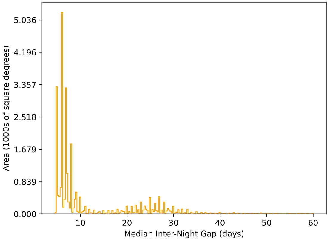
scp_reweight_v3.3_10yrs All sky r band: Median Inter-Night Gap
