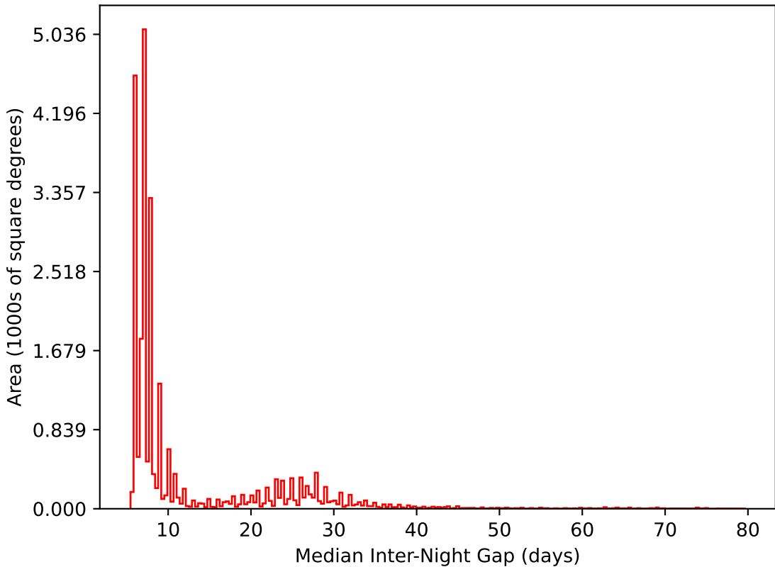
scp_reweight_v3.3_10yrs All sky i band: Median Inter-Night Gap
