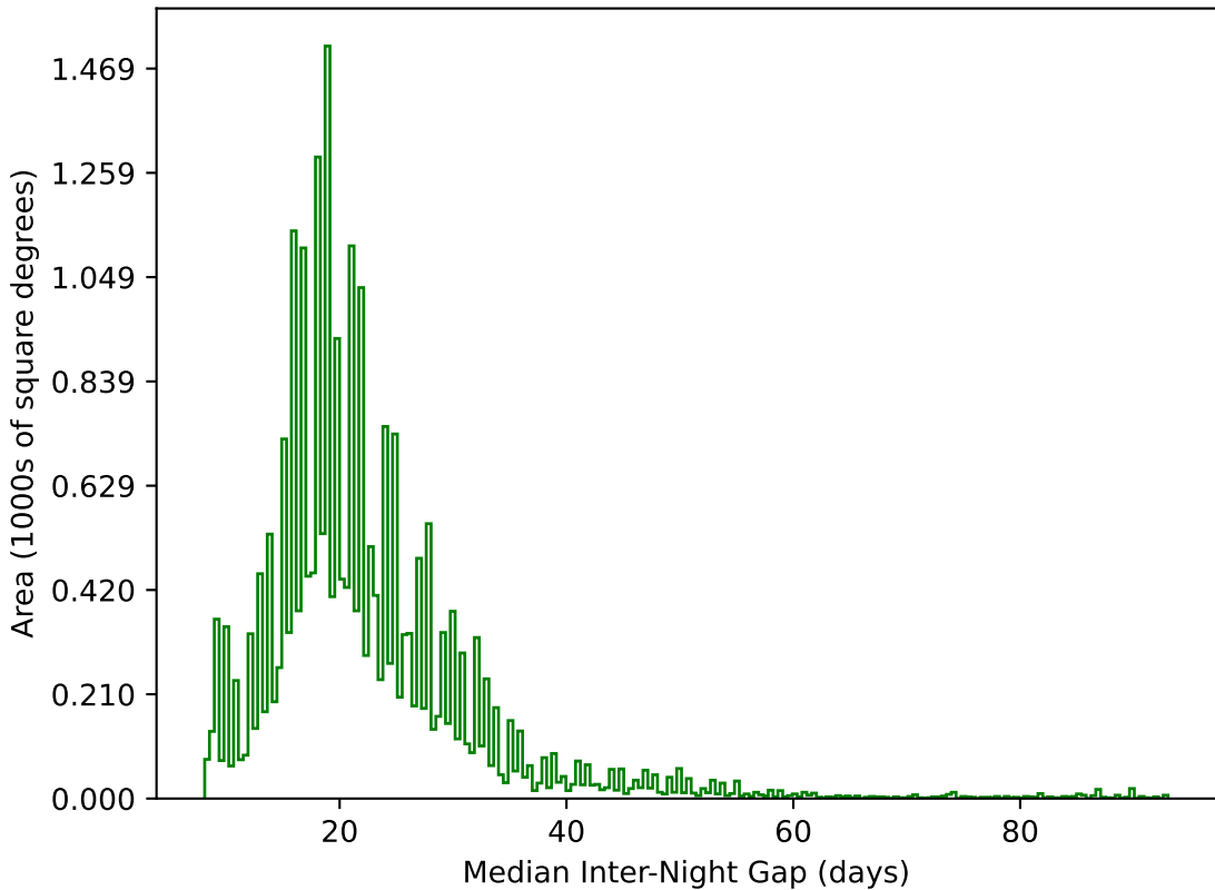
scp_reweight_v3.3_10yrs All sky g band: Median Inter-Night Gap
