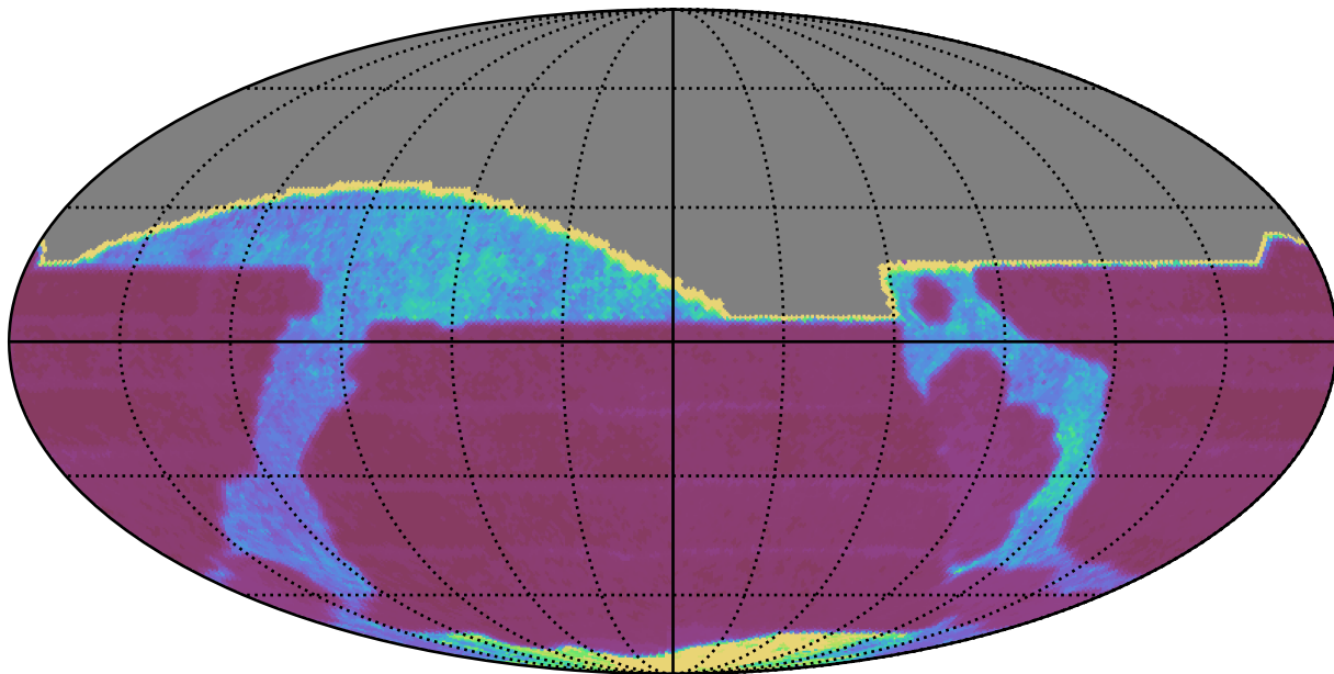
scp_reweight_v3.3_10yrs All sky all bands: Median Inter-Night Gap
