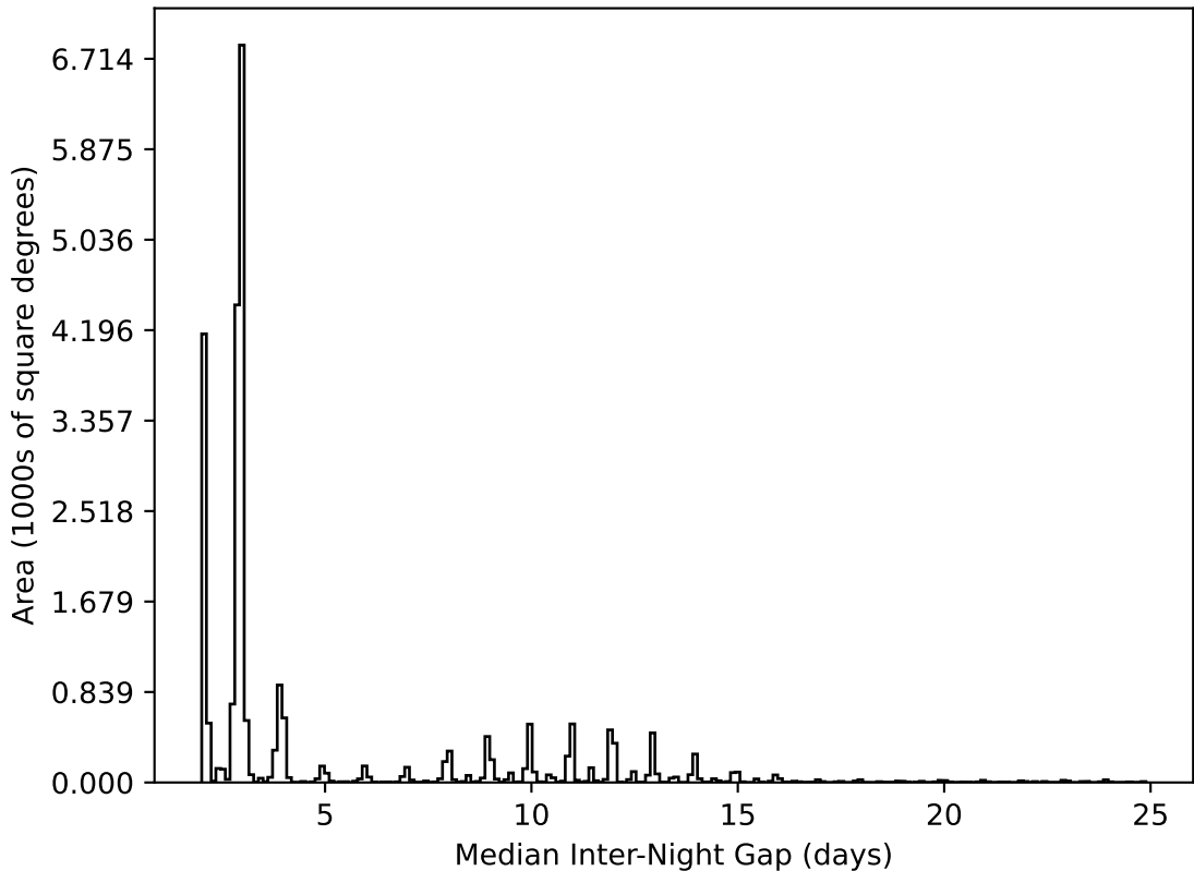
scp_reweight_v3.3_10yrs All sky all bands: Median Inter-Night Gap
