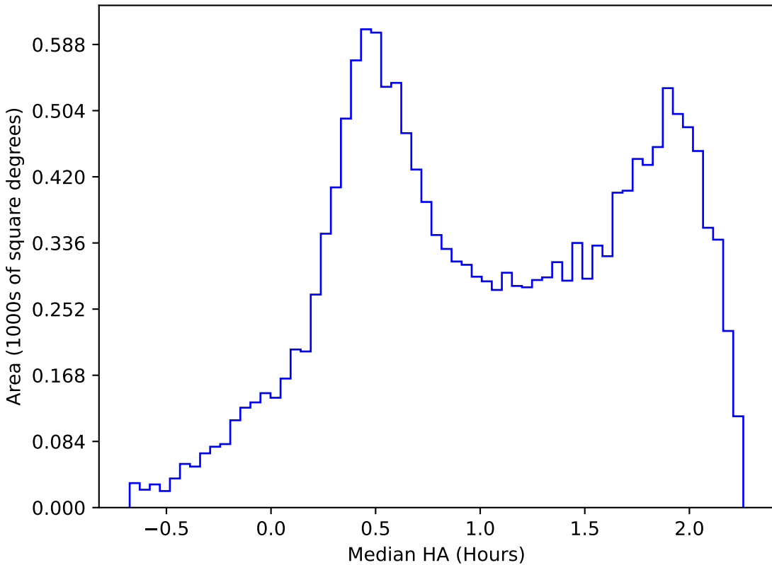
scp_reweight_v3.3_10yrs WFD z band: Median HA
