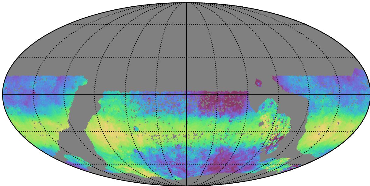
scp_reweight_v3.3_10yrs WFD y band: Median HA
