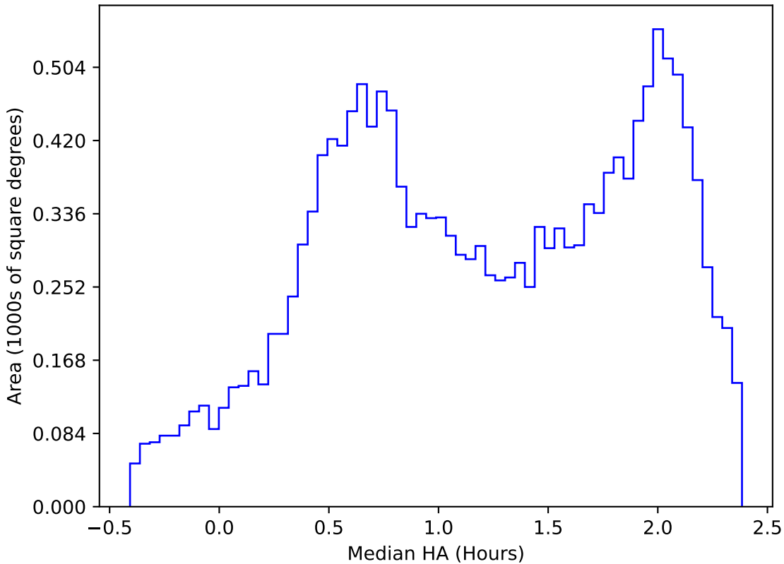
scp_reweight_v3.3_10yrs WFD y band: Median HA
