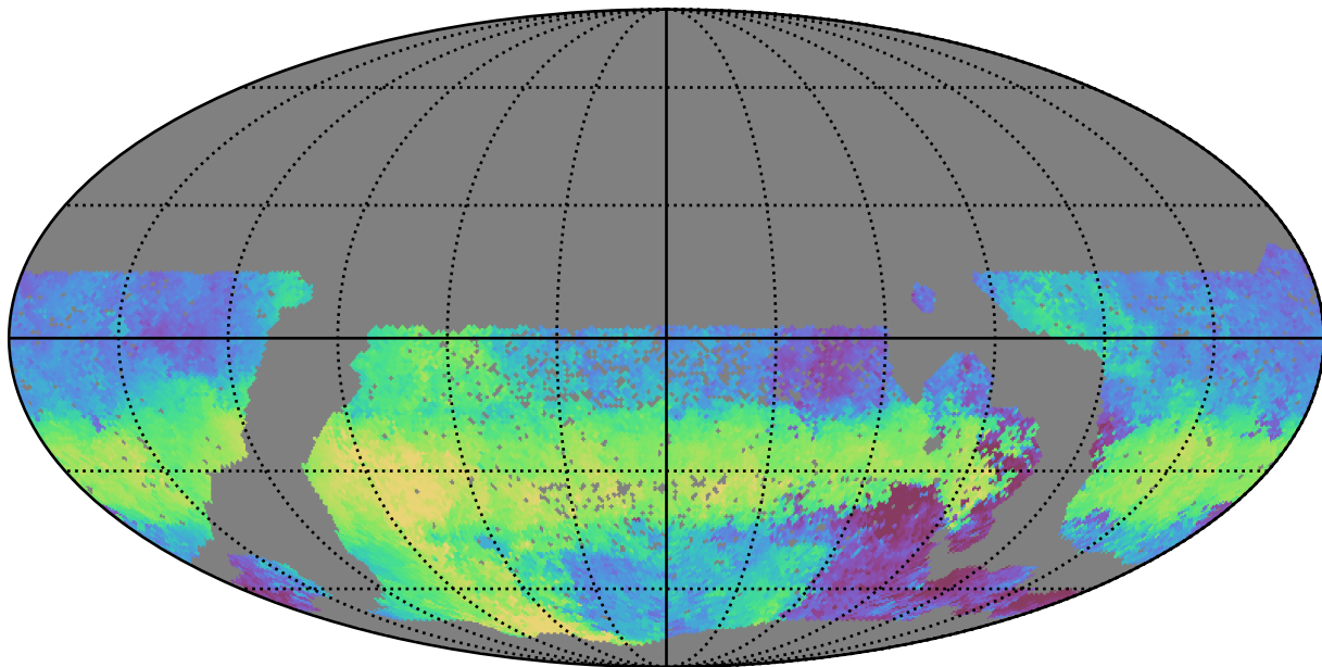
scp_reweight_v3.3_10yrs WFD u band: Median HA
