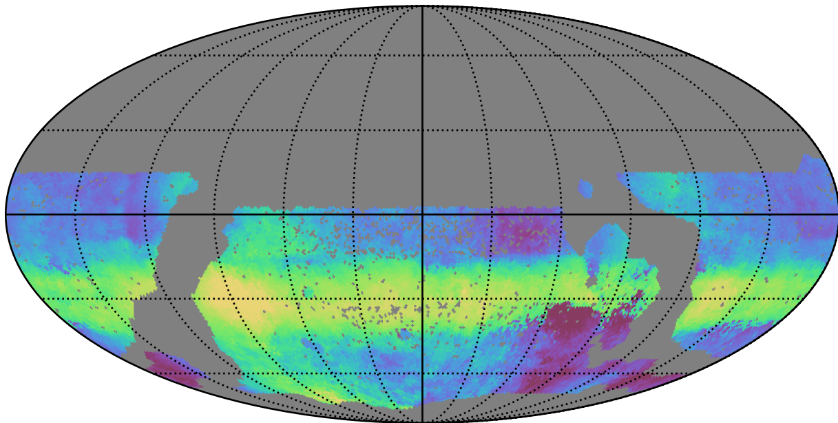
scp_reweight_v3.3_10yrs WFD r band: Median HA
