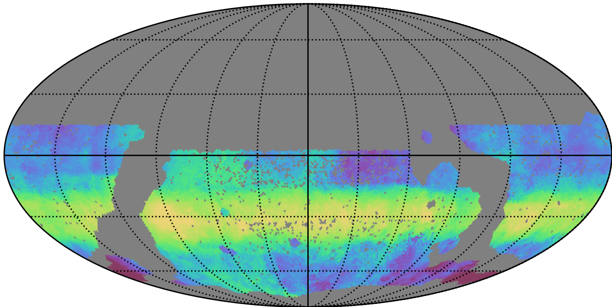
scp_reweight_v3.3_10yrs WFD i band: Median HA
