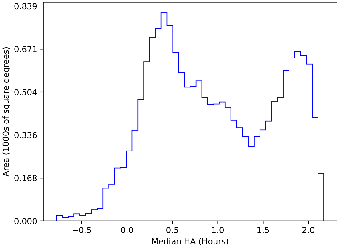
scp_reweight_v3.3_10yrs WFD i band: Median HA
