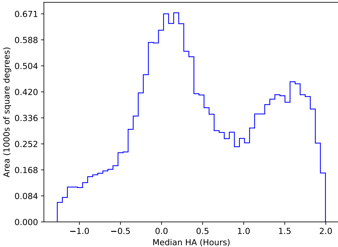
scp_reweight_v3.3_10yrs WFD g band: Median HA
