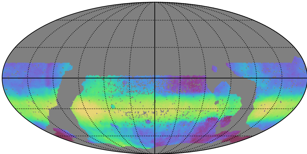
scp_reweight_v3.3_10yrs WFD all bands: Median HA
