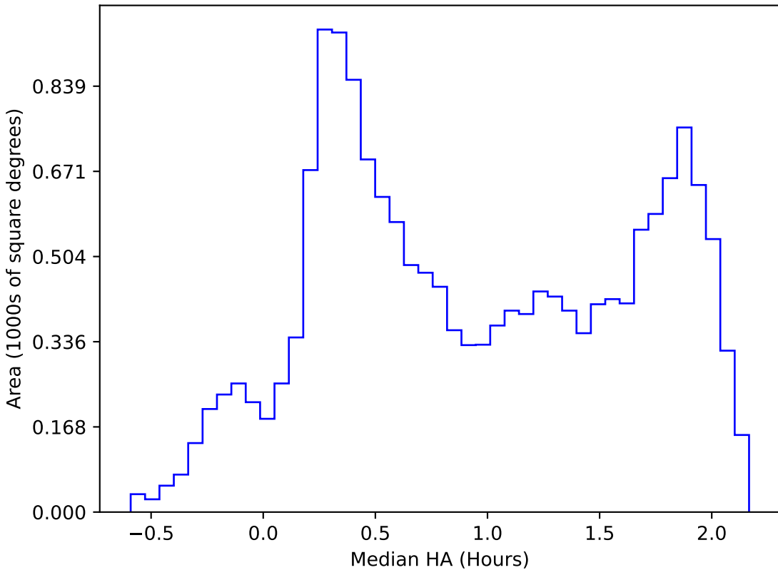
scp_reweight_v3.3_10yrs WFD all bands: Median HA
