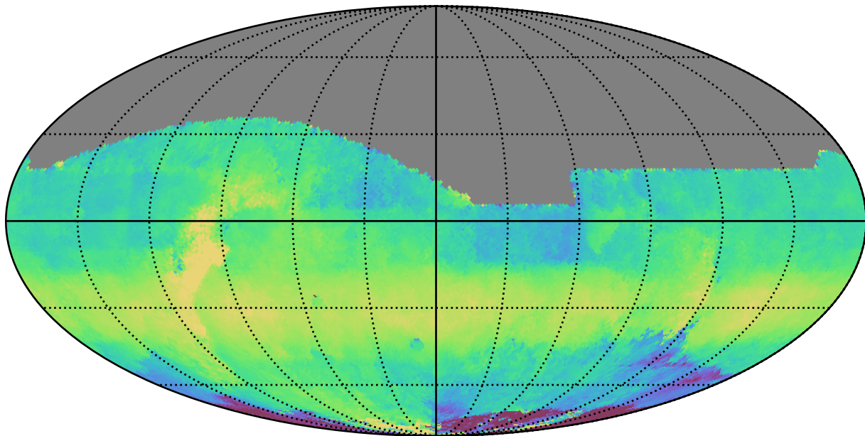
scp_reweight_v3.3_10yrs All sky z band: Median HA
