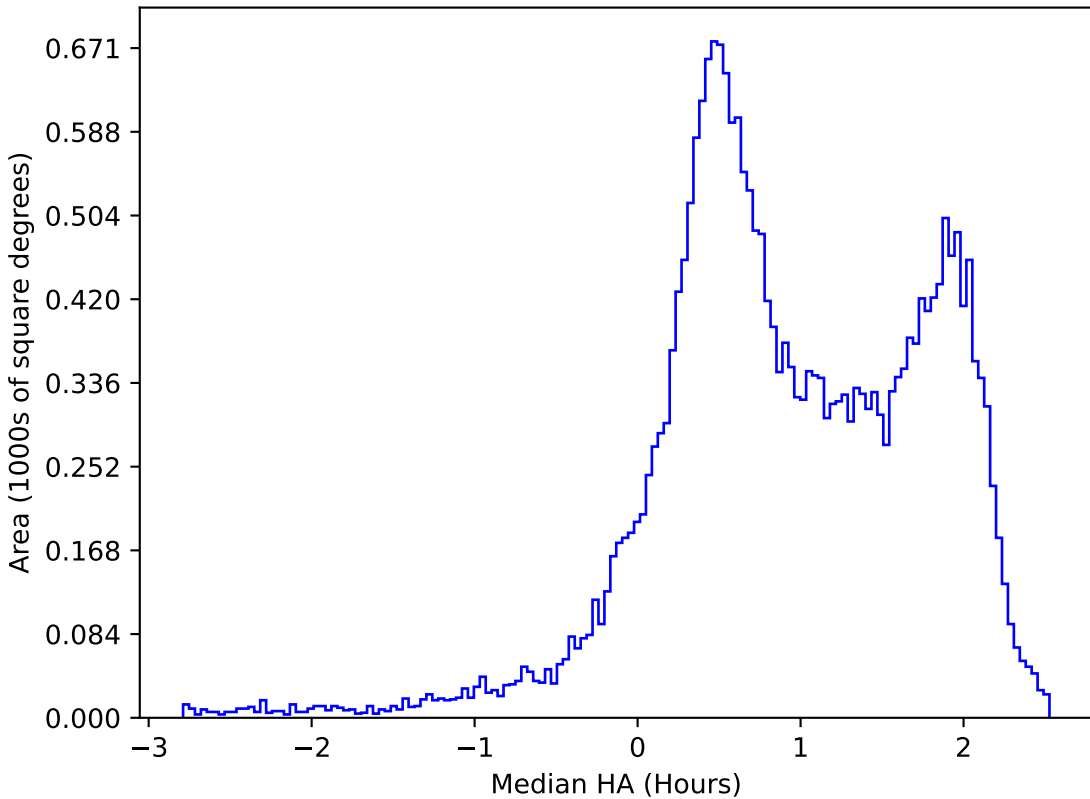
scp_reweight_v3.3_10yrs All sky z band: Median HA
