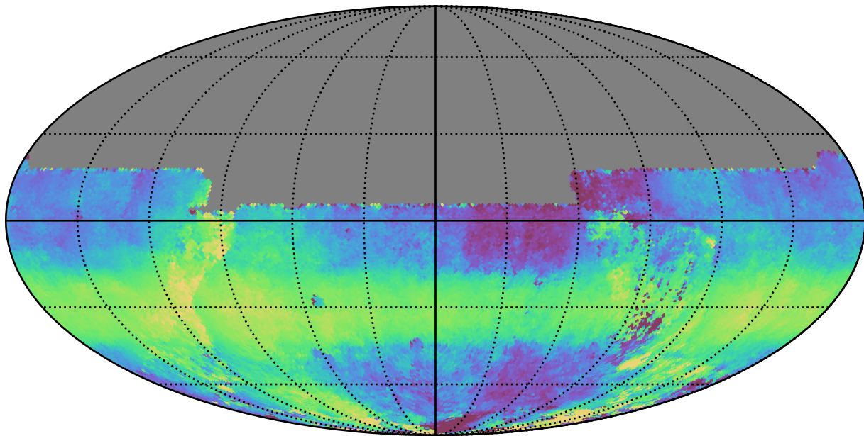
scp_reweight_v3.3_10yrs All sky y band: Median HA
