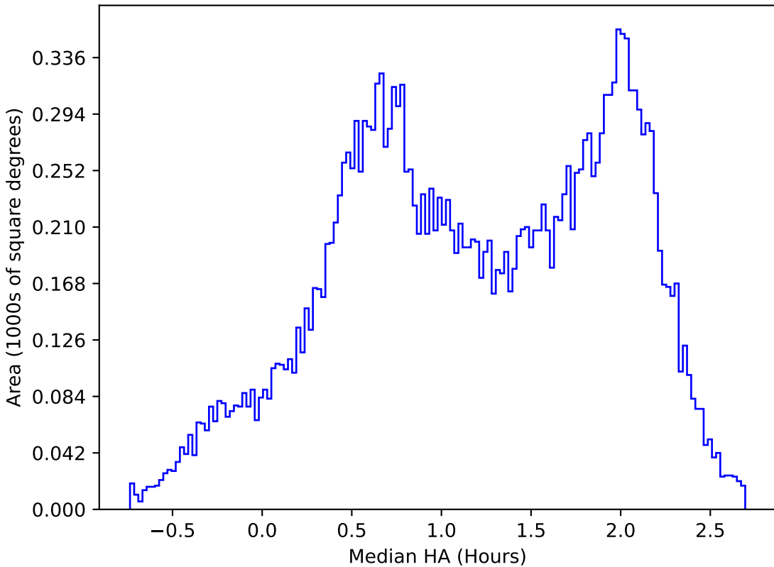
scp_reweight_v3.3_10yrs All sky y band: Median HA
