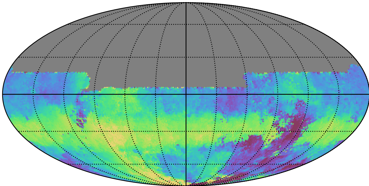
scp_reweight_v3.3_10yrs All sky u band: Median HA
