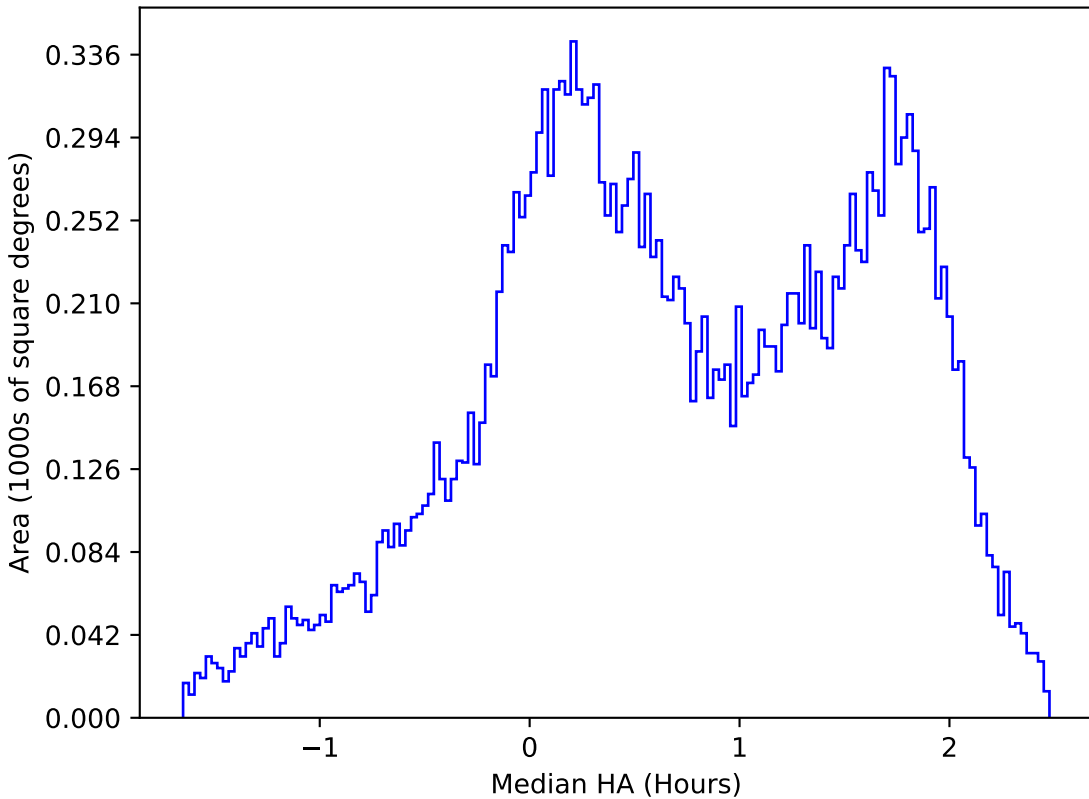
scp_reweight_v3.3_10yrs All sky u band: Median HA
