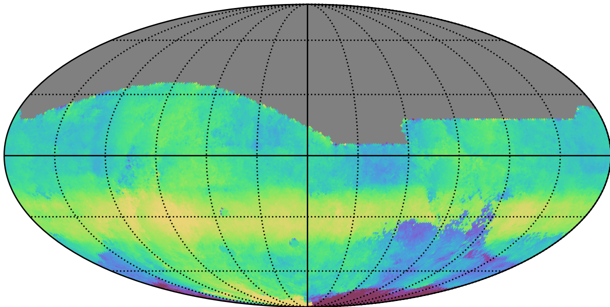
scp_reweight_v3.3_10yrs All sky r band: Median HA
