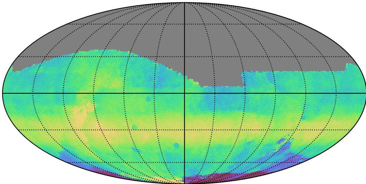
scp_reweight_v3.3_10yrs All sky i band: Median HA
