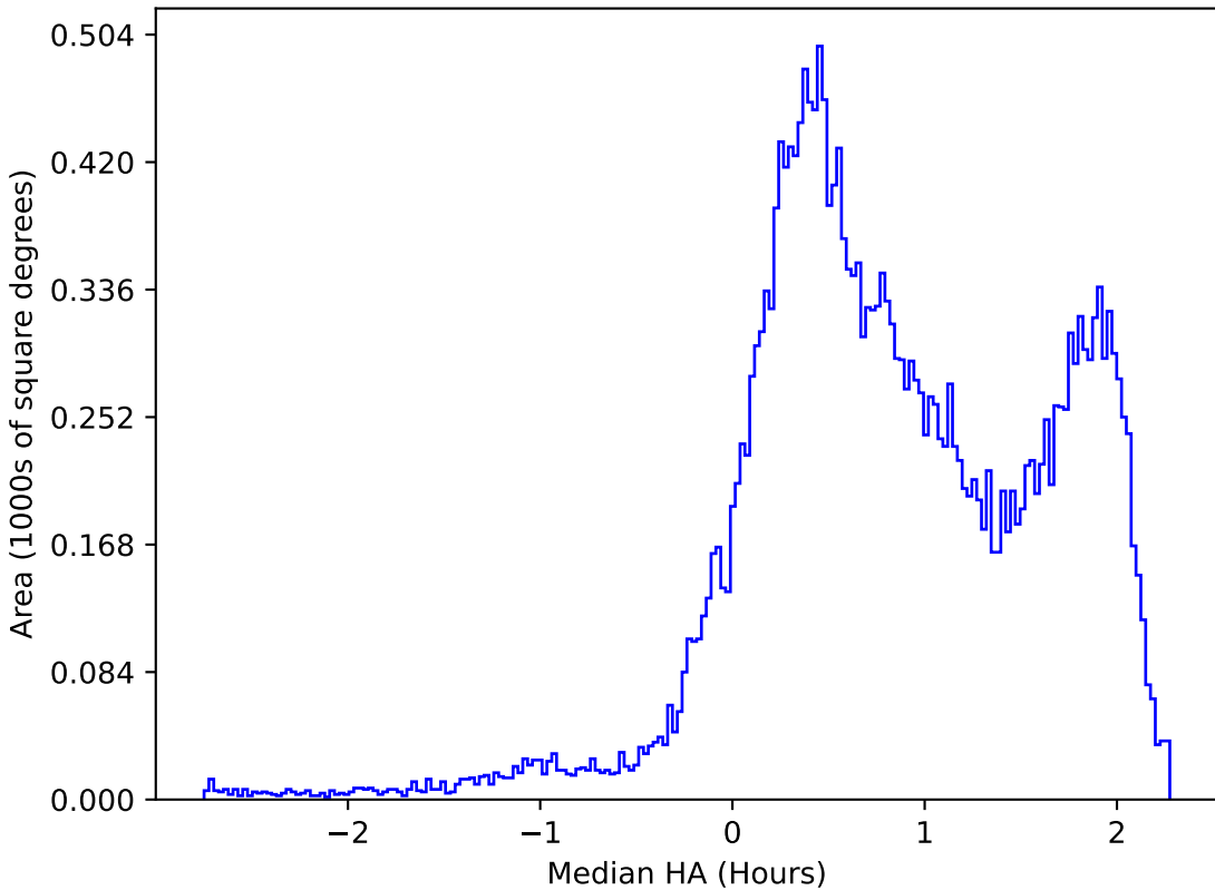
scp_reweight_v3.3_10yrs All sky i band: Median HA
