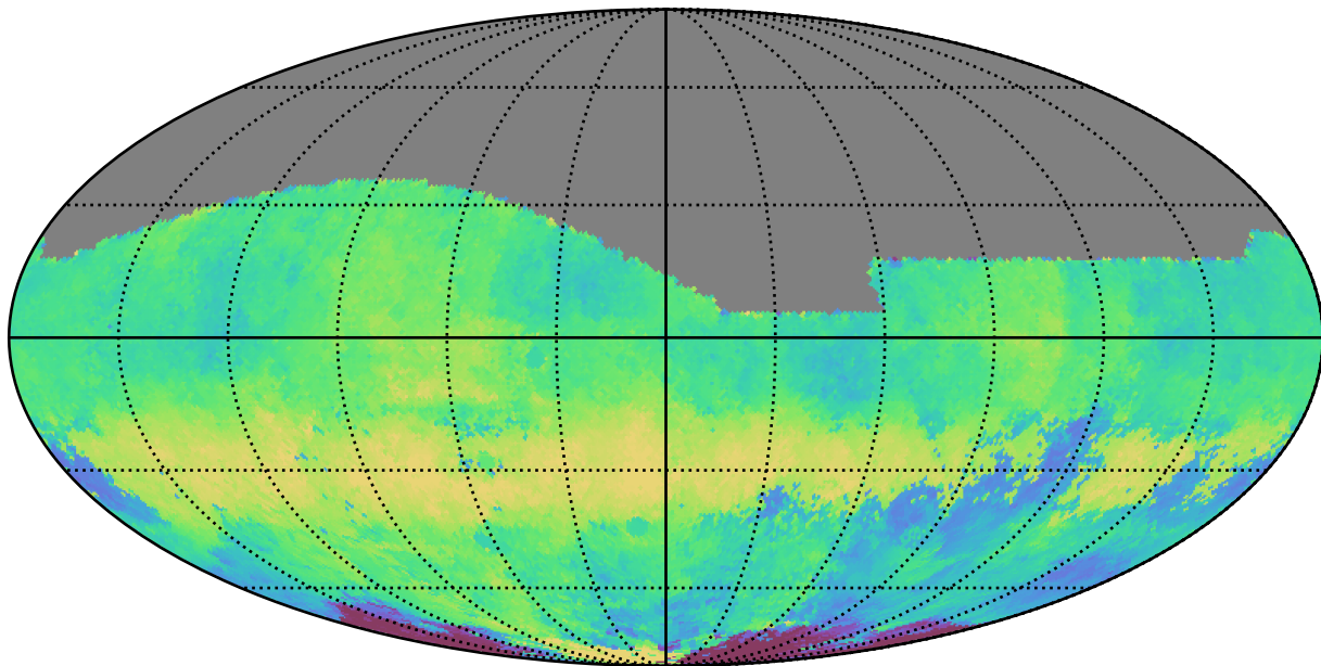
scp_reweight_v3.3_10yrs All sky g band: Median HA
