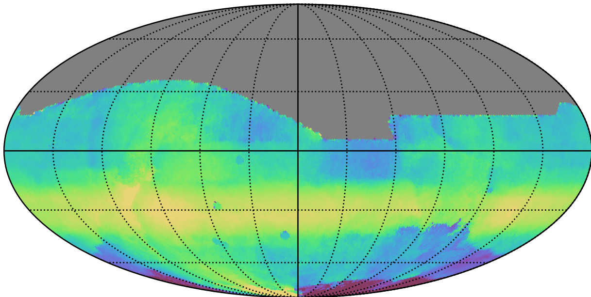
scp_reweight_v3.3_10yrs All sky all bands: Median HA
