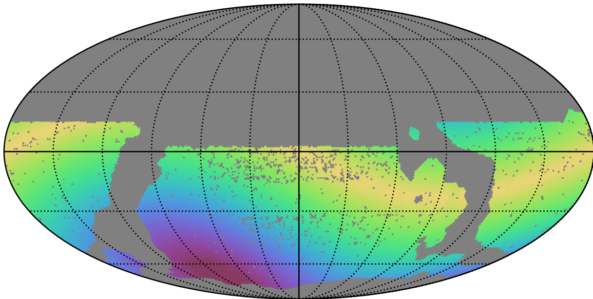
scp_reweight_v3.3_10yrs WFD z band: Max solarElong
