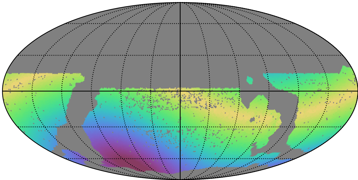
scp_reweight_v3.3_10yrs WFD y band: Max solarElong
