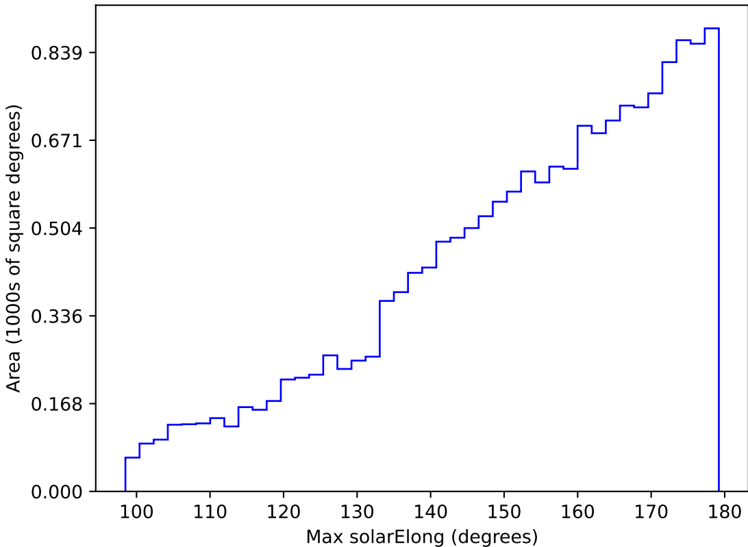
scp_reweight_v3.3_10yrs WFD y band: Max solarElong
