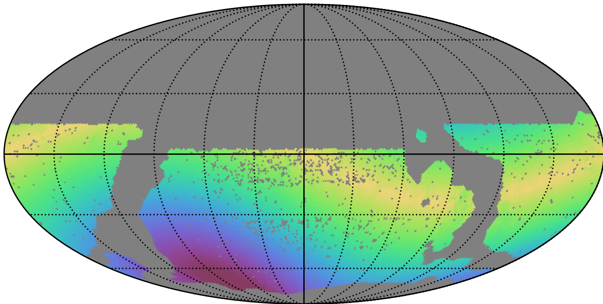
scp_reweight_v3.3_10yrs WFD u band: Max solarElong
