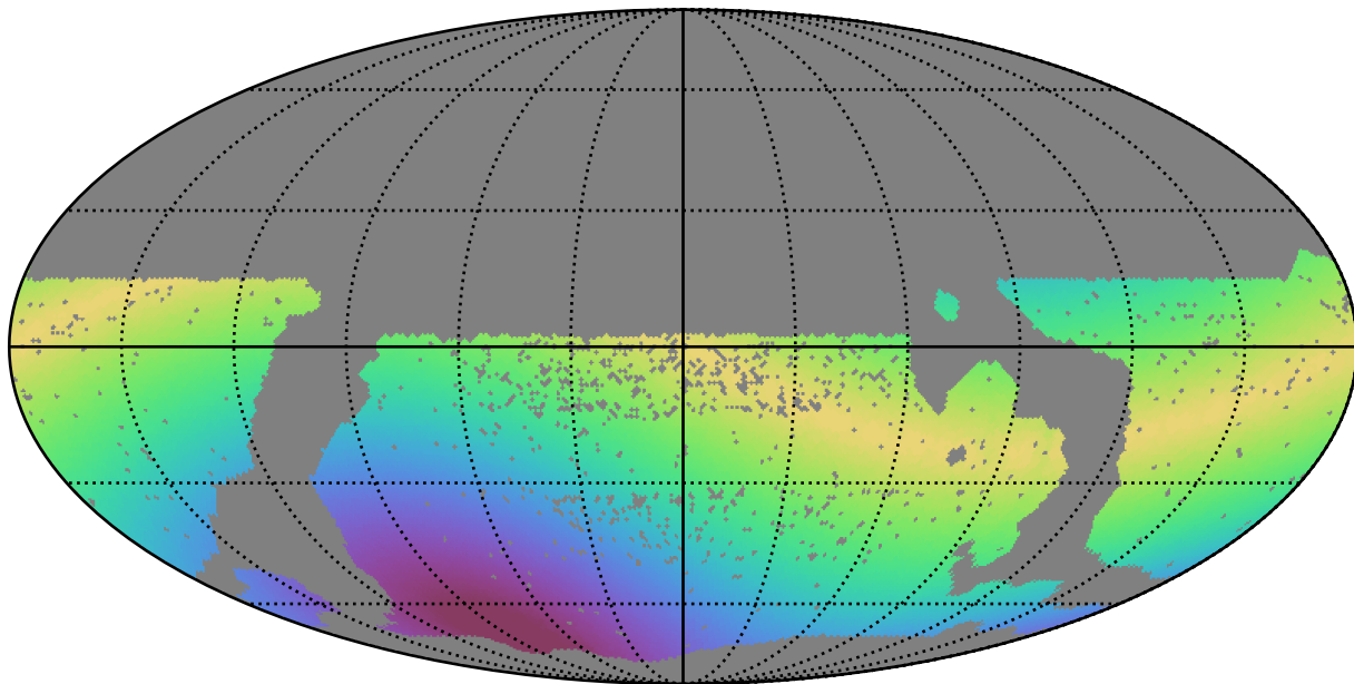
scp_reweight_v3.3_10yrs WFD r band: Max solarElong
