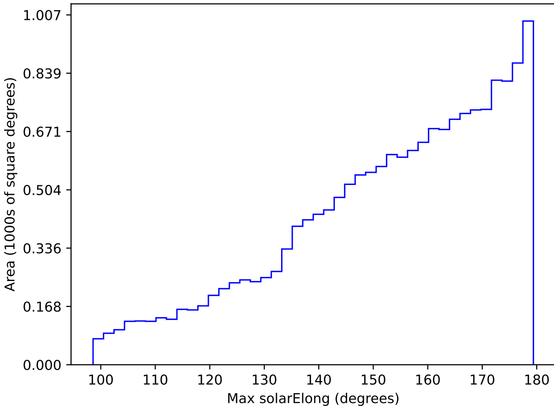
scp_reweight_v3.3_10yrs WFD r band: Max solarElong
