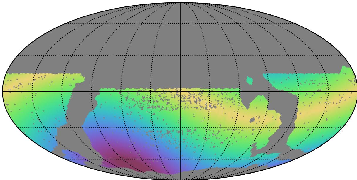
scp_reweight_v3.3_10yrs WFD i band: Max solarElong
