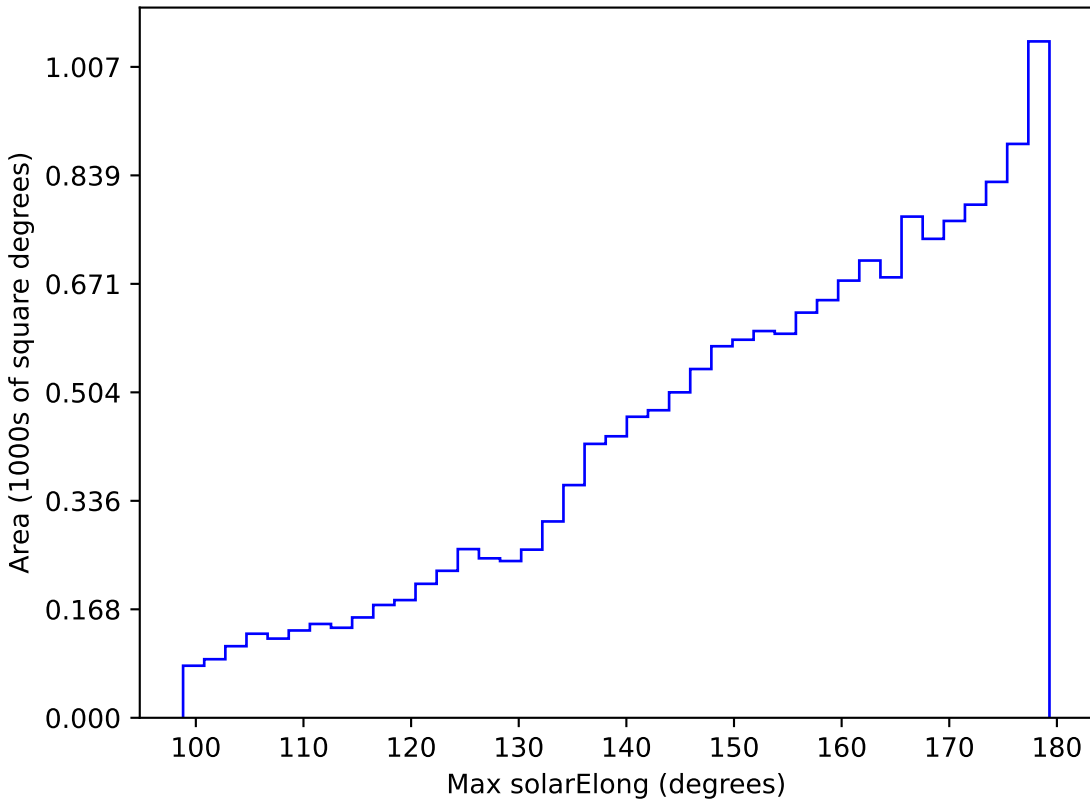
scp_reweight_v3.3_10yrs WFD i band: Max solarElong
