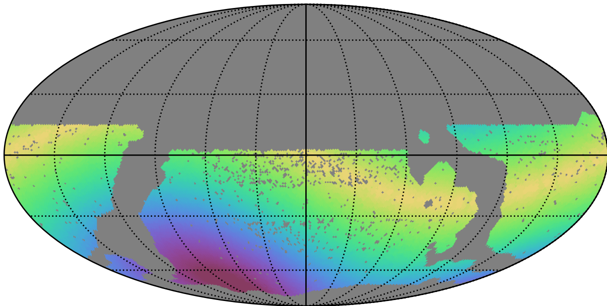
scp_reweight_v3.3_10yrs WFD g band: Max solarElong
