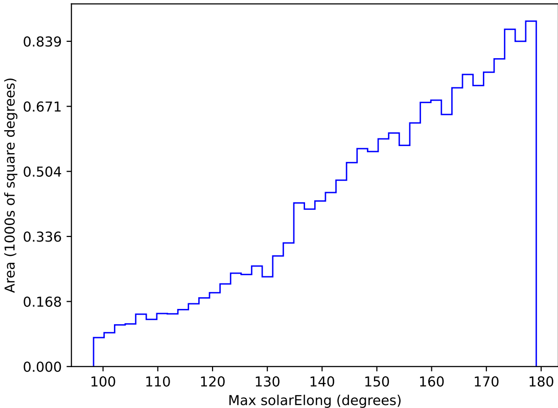
scp_reweight_v3.3_10yrs WFD g band: Max solarElong
