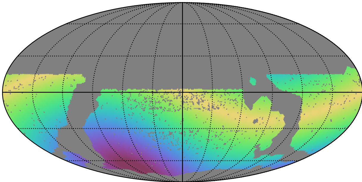
scp_reweight_v3.3_10yrs WFD all bands: Max solarElong
