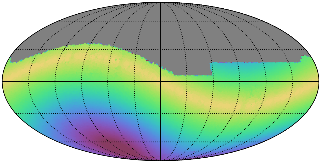
scp_reweight_v3.3_10yrs All sky z band: Max solarElong
