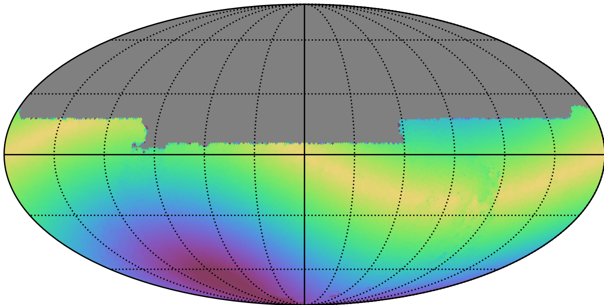
scp_reweight_v3.3_10yrs All sky y band: Max solarElong
